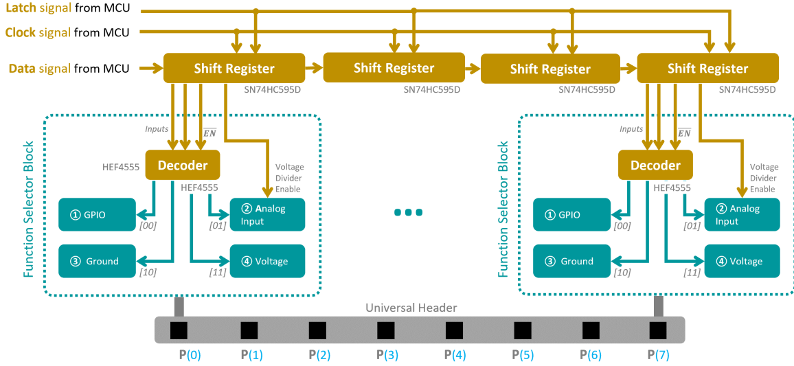
Fig. 10. Block diagram of all components required for changing the assignments of the programmable header pins of the CircuitGlue board.
