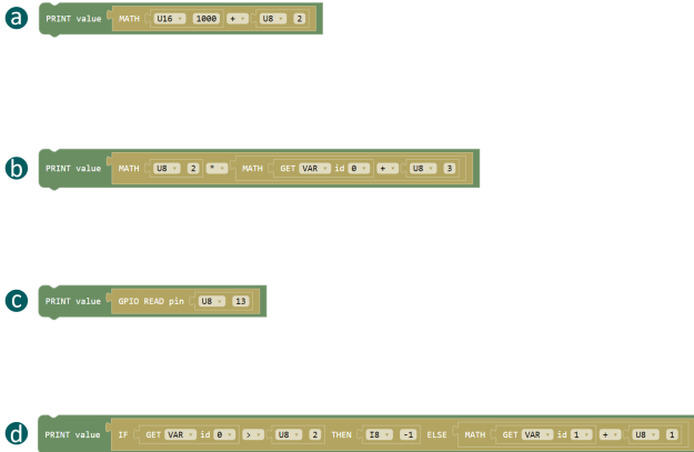
LogicGlue Visual Block-based Interface
